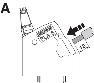
Functional drawing
