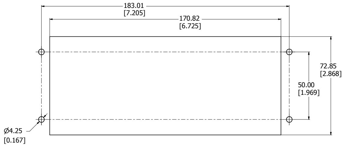
MOUNTING OPENING
