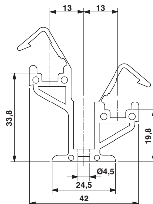
Dimensional drawing
