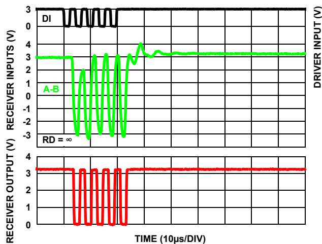
FIGURE 29. ISL32602E, ISL32603E PERFORMANCE WITH V_{CC} = 3.3V , 460kbps, 2000ft (610m) CAT 5 CABLE
