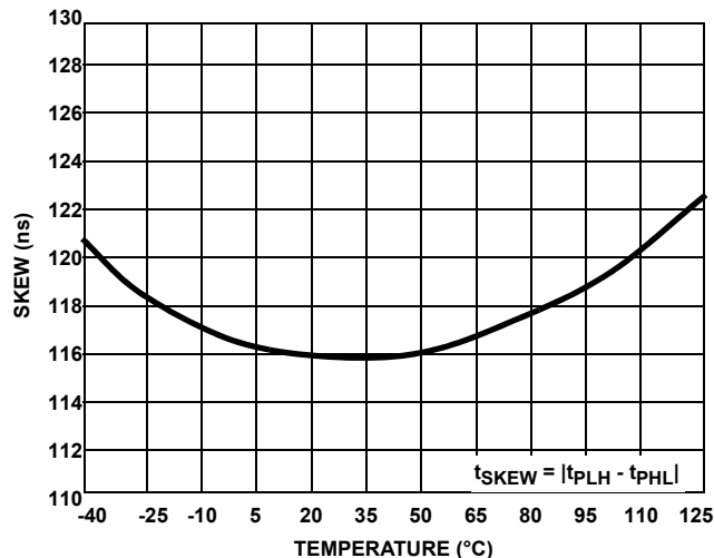
FIGURE 19. ISL32600E, ISL32601E RECEIVER SKEW vs TEMPERATURE
