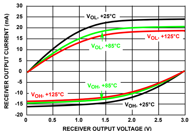
FIGURE 11. ISL32600E, ISL32601E RECEIVER OUTPUT CURRENT vs RECEIVER OUTPUT VOLTAGE
