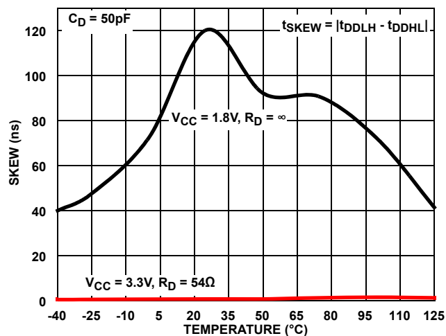
FIGURE 31. ISL32602E, ISL32603E DRIVER DIFFERENTIAL SKEW vs TEMPERATURE
