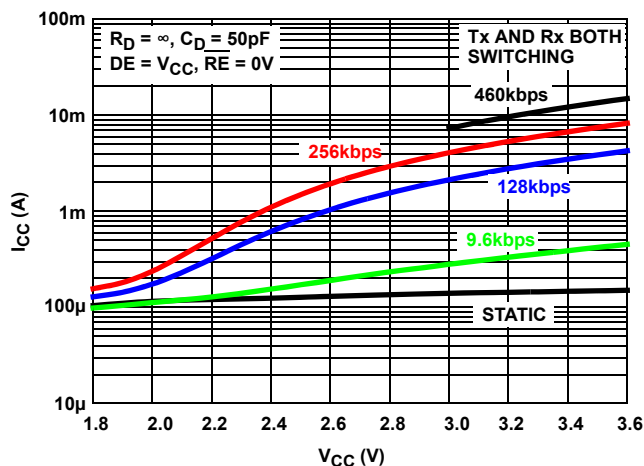
FIGURE 27. ISL32602E, ISL32603E DYNAMIC SUPPLY CURRENT vs SUPPLY VOLTAGE AT DIFFERENT DATA RATES
