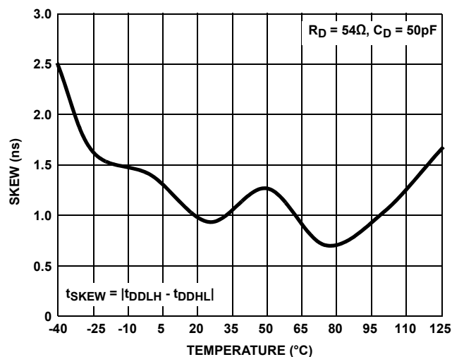
FIGURE 17. ISL32600E, ISL32601E DRIVER DIFFERENTIAL SKEW vs TEMPERATURE
