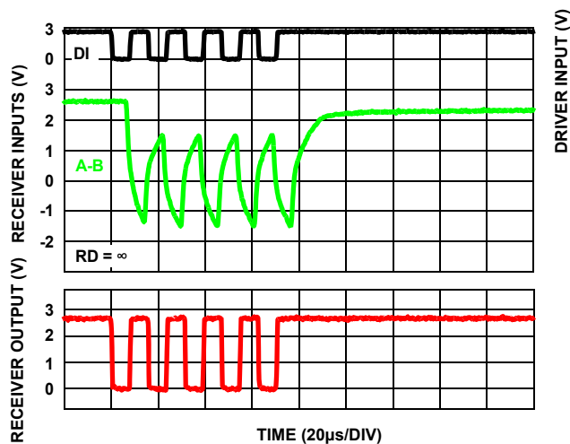
FIGURE 15. ISL32600E, ISL32601E PERFORMANCE WITH V_{CC} = 2.7V , 128kbps, 4000ft (1220m) CAT 5 CABLE
