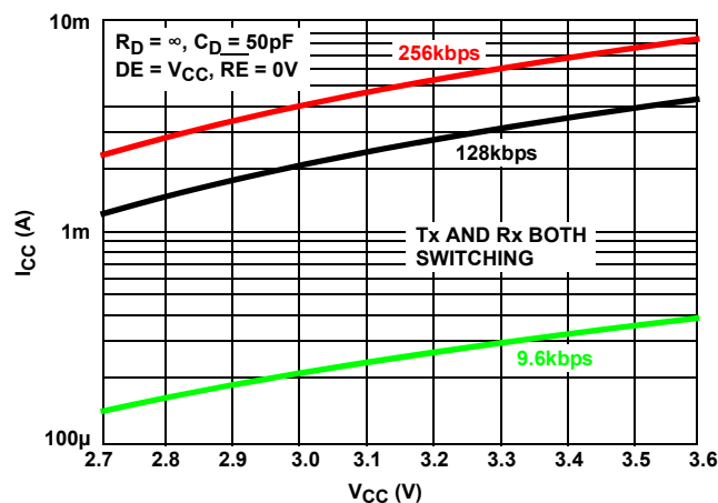
FIGURE 13. ISL32600E, ISL32601E DYNAMIC SUPPLY CURRENT vs SUPPLY VOLTAGE AT DIFFERENT DATA RATES
