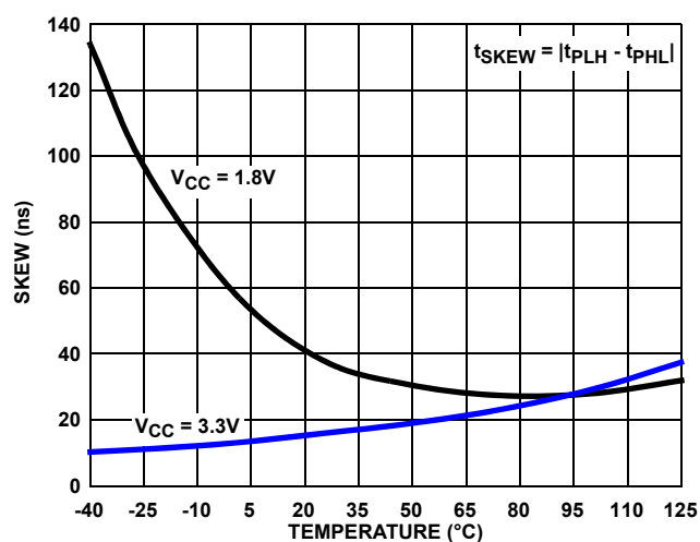
FIGURE 33. ISL32602E, ISL32603E RECEIVER SKEW vs TEMPERATURE
