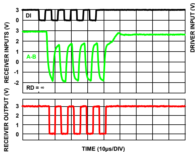
FIGURE 14. ISL32600E, ISL32601E PERFORMANCE WITH V_{CC} = 3V , 256kbps, 3000ft (915m) CAT 5 CABLE
