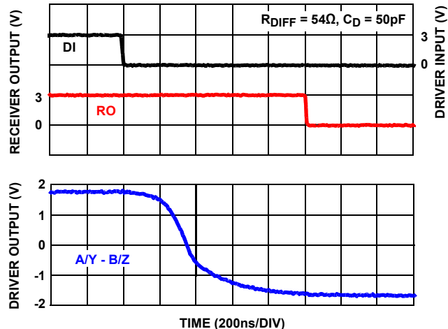
FIGURE 21. ISL32600E, ISL32601E DRIVER AND RECEIVER WAVEFORMS, HIGH TO LOW
