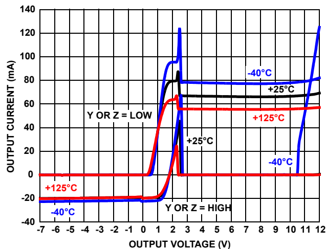
FIGURE 23. ISL32602E, ISL32603E DRIVER OUTPUT CURRENT vs SHORT CIRCUIT VOLTAGE
