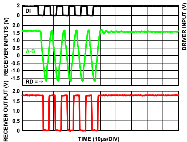
FIGURE 28. ISL32602E, ISL32603E PERFORMANCE WITH V_{CC} = 1.8V , 256kbps, 1000ft (305m) CAT 5 CABLE
