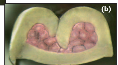
Significant flash can be generated with excessive anvil to crimper clearance, as shown by nominal design condition (a) and +0.003 in over nominal condition (b)
