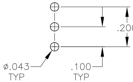
RECOMMENDED PCB LAYOUT TOLERANCES +/- .002
