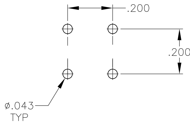
RECOMMENDED PCB LAYOUT TOLERANCES +/- .002
