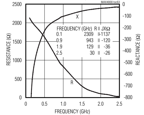
MAX4002 INPUT IMPEDANCE vs. FREQUENCY ( \mu MAX)
