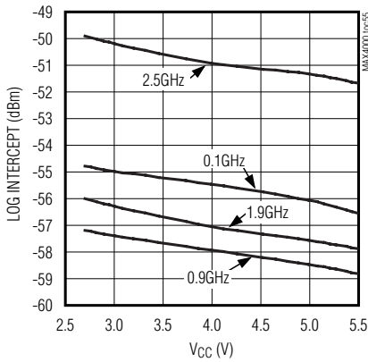
MAX4000 LOG INTERCEPT vs. V_{CC} (UCSP)
