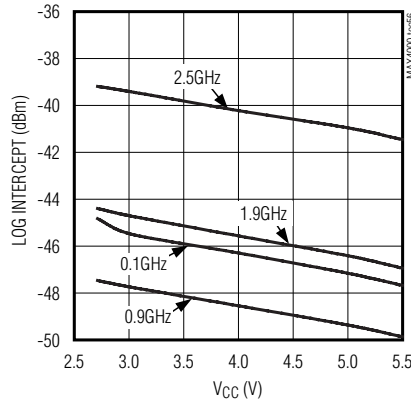
MAX4001 LOG INTERCEPT vs. V_{CC} (UCSP)
