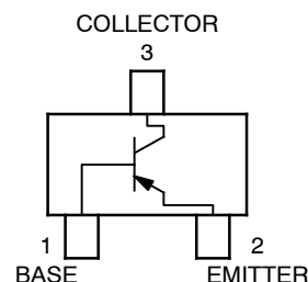
SC-70 (SOT-323) CASE 419 STYLE 3
