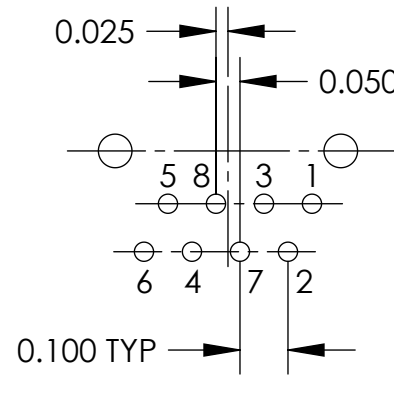
(8 PIN) THRU HOLE TERMINATION TRAPC8M1X TRAPC8MX
