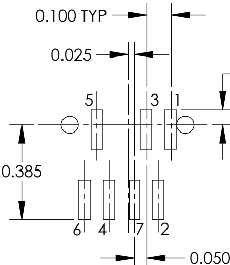
(7 PIN) SURFACE MOUNT TRASM7M1X TRASM7MX
