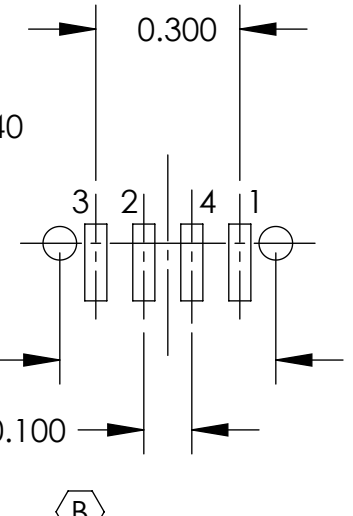
(4 PIN) SMALL PROFILE SURFACE MOUNT TRASM3MS1X TRASM3MSX
