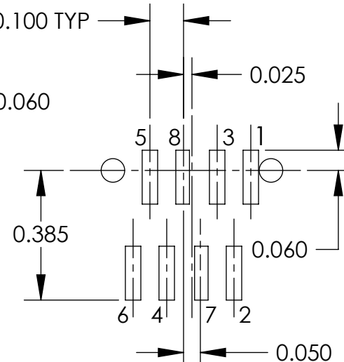
(8 PIN) SURFACE MOUNT TRASM8M1X TRASM8MX
