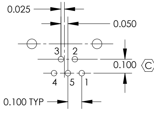
(5 PIN) THRU HOLE TERMINATION TRAPC5M1X TRAPC5MX
