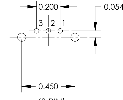
(3 PIN) SMALL PROFILE THRU HOLE TERMINATION TRAPC3MS1X TRAPC3MSX
