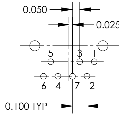
(7 PIN) THRU HOLE TERMINATION TRAPC7M1X TRAPC7MX
