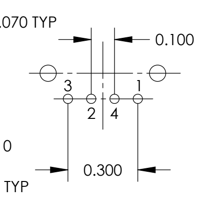
(4 PIN) THRU HOLE TERMINATION TRAPC4M1X TRAPC4MX
