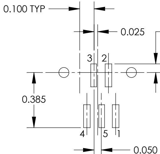
(5 PIN) SURFACE MOUNT TRASM5M1X TRASM5MX
