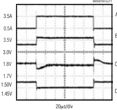
3A LOAD TRANSIENT (IRF7401)
