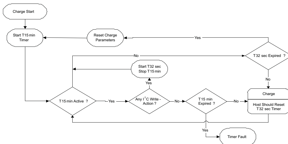
Figure 17. Timer Flow Chart for bq24153A/6A/8/9
