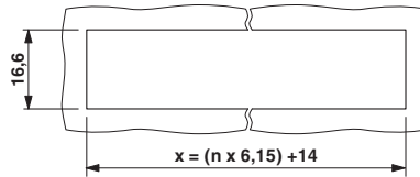
Dimensional drawing
