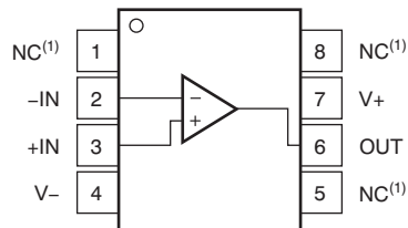
OPA171 D Package 8-Pin SOIC Top View
