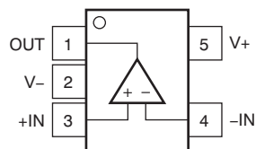
OPA171 DBV Package 5-Pin SOT-23 Top View
