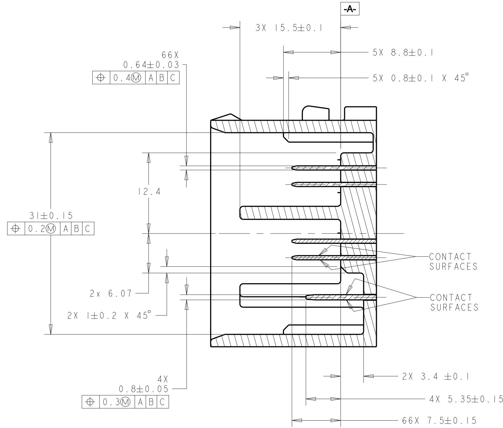
SECTION C-C
