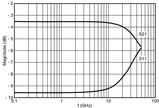
CH0402 wraparound ( Z_0 = Z_l = Z_s = R = 50 \Omega )
