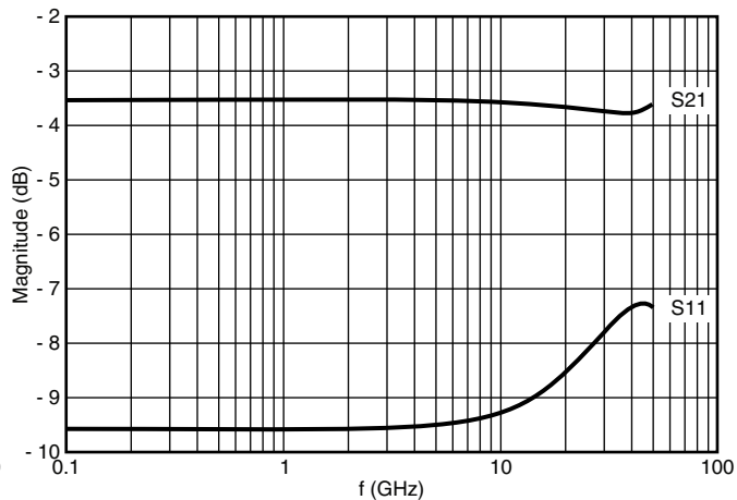
CH0402 wraparound ( Z_0 = Z_l = Z_s = R = 100 \Omega )
