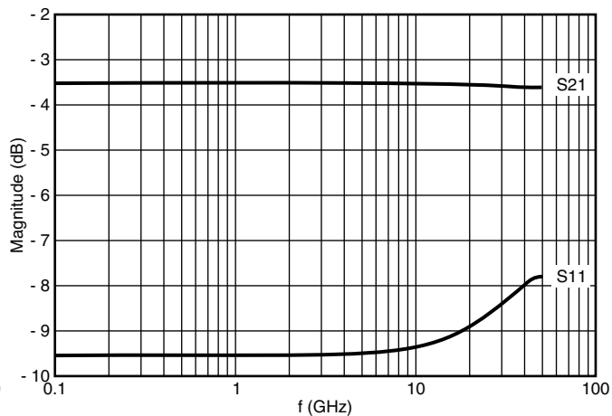
CH0402 flip chip ( Z_0 = Z_l = Z_s = R = 100 \Omega )
