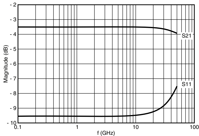
CH0402 flip chip ( Z_0 = Z_l = Z_s = R = 50 \Omega )
