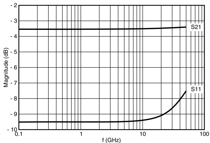
CH02016 flip chip ( Z_0 = Z_l = Z_s = R = 100 \Omega )
