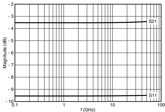
CH02016 flip chip ( Z_0 = Z_l = Z_s = R = 50 \Omega )
