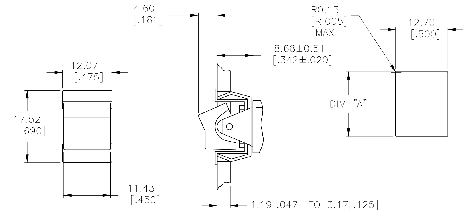
J50 SNAP-IN
