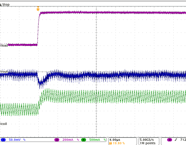
Figure 36. PWM-to-PSM Transition
