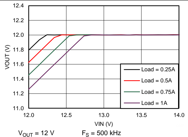
Figure 74. Dropout Curve
