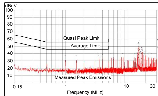
Figure 24. Conducted EMI Curve Measured on LM46001PWPEVM with L = 27\text{ }\mu\text{H} , C_{OUT} = 66\text{ }\mu\text{F} , C_{FF} = 33\text{ pF} . EVM input filter L_{in} = 1\text{ }\mu\text{H} , C_d = 47\text{ }\mu\text{F} , C_{IN4} = 68\text{ }\mu\text{F}
