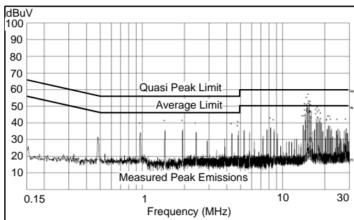
Figure 23. Conducted EMI Curve Measured on LM46001PWPEVM with default BOM. EVM input filter: L_{in} = 1\text{ }\mu\text{H} , C_d = 47\text{ }\mu\text{F} , C_{IN4} = 68\text{ }\mu\text{F}
