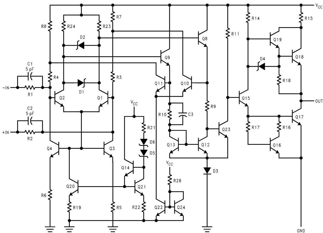
Figure 2. Equivalent Circuit
