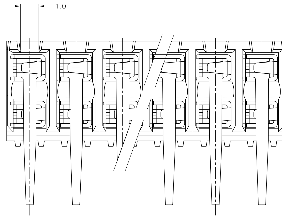
REAR VIEW
