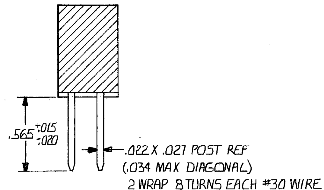
SECTION A-A WRAP-TYPE CONTACT (TYPE V) PC MOUNT
