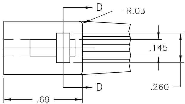
VIEW C-C
