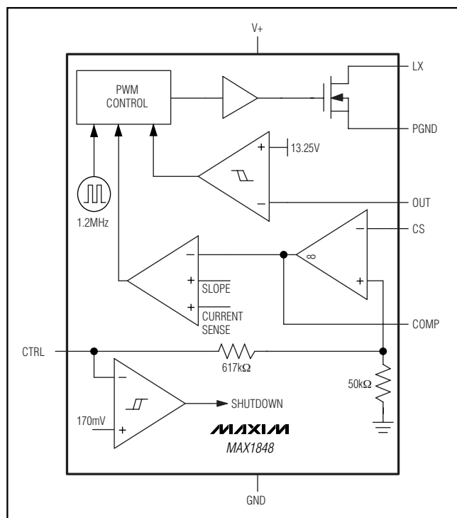
Figure 1. Functional Diagram
