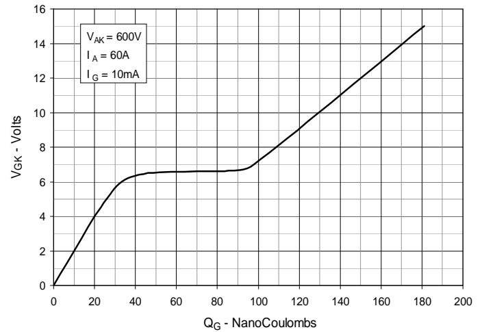
Fig. 4. Gate Charge
