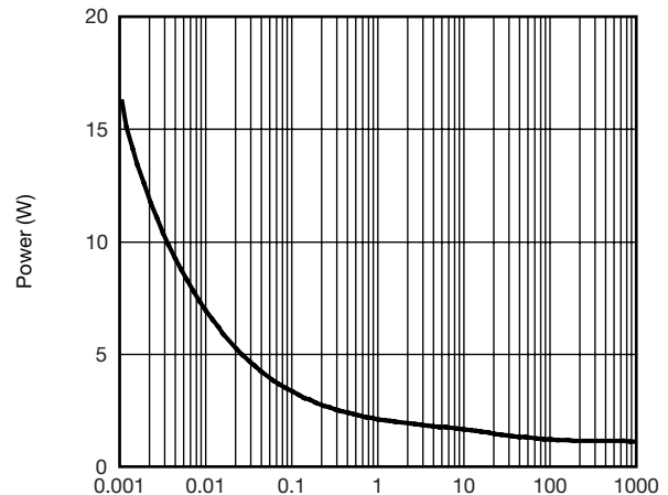
Power (W) Single Pulse Power, Junction-to-Ambient
