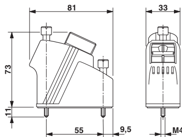
Dimensional drawing
