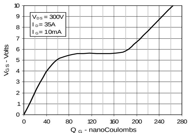
Fig. 10. Gate Charge
