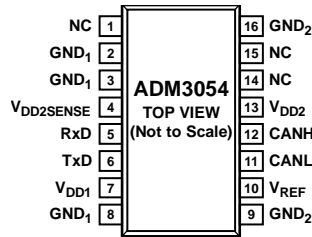
Figure 2. Pin Configuration
