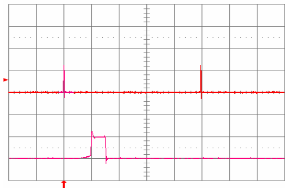
Fig. 2.5V.18: Load current (top trace, 20 A/div., 20 ms/div.) into a 10 m\Omega short circuit during restart, at V_{in} = 48 V. Bottom trace (20 A/div., 1 ms/div.) is an expansion of the on-time portion of the top trace.
