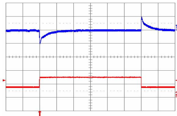
Fig. 3.3V.12: Output voltage response to load current step-change (3.75 A – 7.5 A – 3.75 A) at V_{in} = 48 V. Top trace: output voltage (100 mV/div.). Bottom trace: load current (5 A/div.). Current slew rate: 5 A/ \mu s. C_o = 450 \mu F tantalum + 1 \mu F ceramic. Time scale: 0.2 ms/div.
