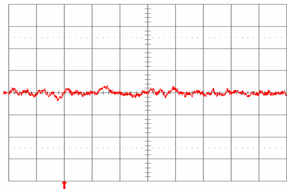
Fig. 2.5V.16: Input reflected ripple current, i_s (10 mA/div.), measured through 10 \mu H at the source at full rated load current and V_{in} = 48 V. Refer to Fig. 2.5V.14 for test setup. Time scale: 1 \mu s/div.
