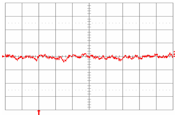
Fig. 1.8V.16: Input reflected ripple current, i_s (10 mA/div.), measured through 10 \mu H at the source at full rated load current and V_{in} = 48 V. Refer to Fig. 1.8V.14 for test setup. Time scale: 1 \mu s/div.
