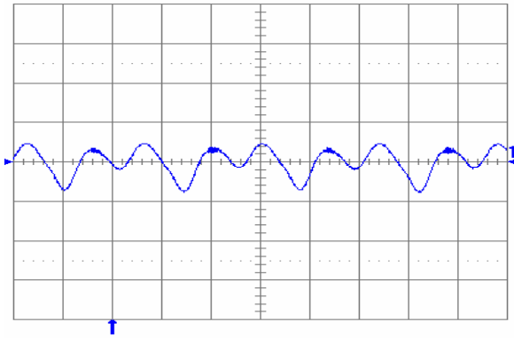
Fig. 1.5V.13: Output voltage ripple (20 mV/div.) at full rated load current into a resistive load with C_o = 10 μF tantalum + 1 μF ceramic and V_{in} = 48 V. Time scale: 1 μs/div.
