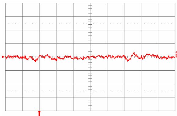
Fig. 1.2V.16: Input reflected ripple current, i_s (10 mA/div.), measured through 10 \mu H at the source at full rated load current and V_{in} = 48 V. Refer to Fig. 1.2V.14 for test setup. Time scale: 1 \mu s/div.
