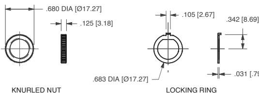
LOCKING RING
