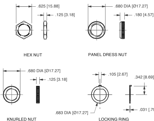
LOCKING RING
