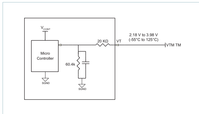
Figure 30 — VT Connections
