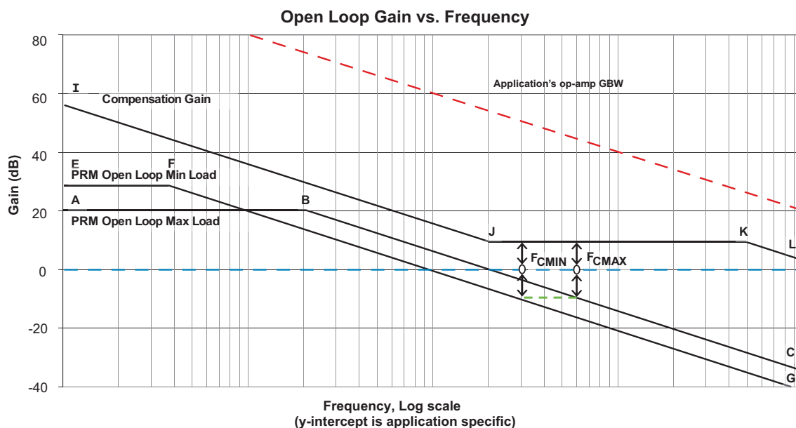
Figure 38 — Reference asymptotic Bode plot for the considered system
