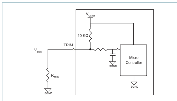
Figure 25 — TRIM Connection
