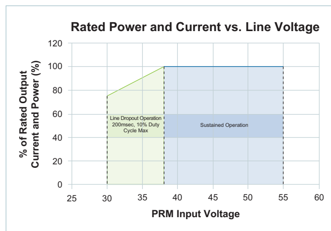
Figure 42 — Line Dropout Derating
