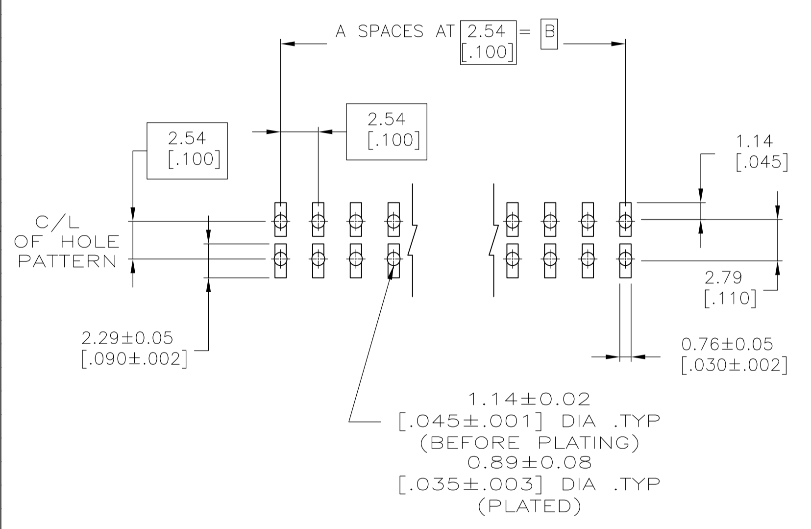
RECOMMENDED PC BOARD MOUNTING DIMENSIONS FOR .063 [1.60] THICK PC BOARD AND .012 [0.305] STENCIL THICK.
