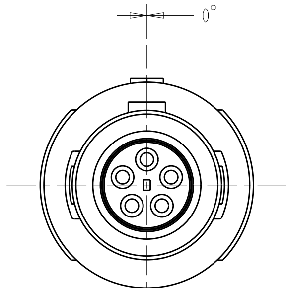
0° KEYING SCALE 4:1
