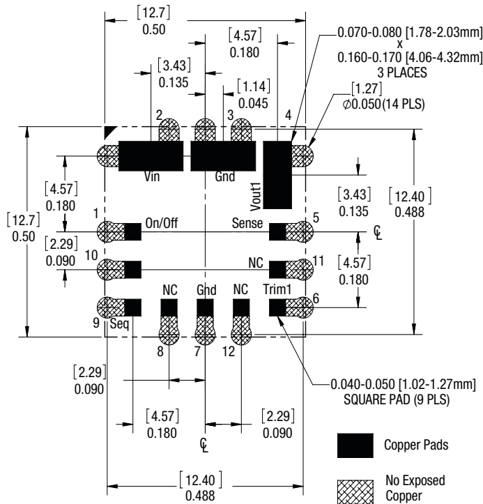
Figure 3. OKL-T/6-W5 Mechanical Outline
