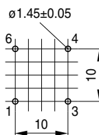
Recommended hole arrangement (view in mounting direction)
