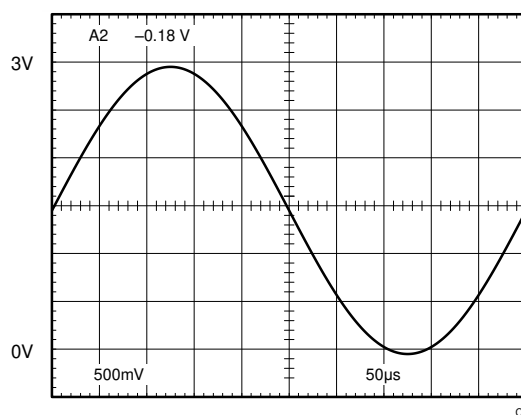
Rail-to-Rail Output
