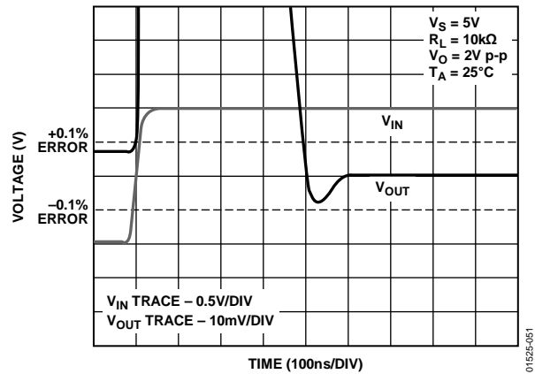
Figure 51. Settling Time
