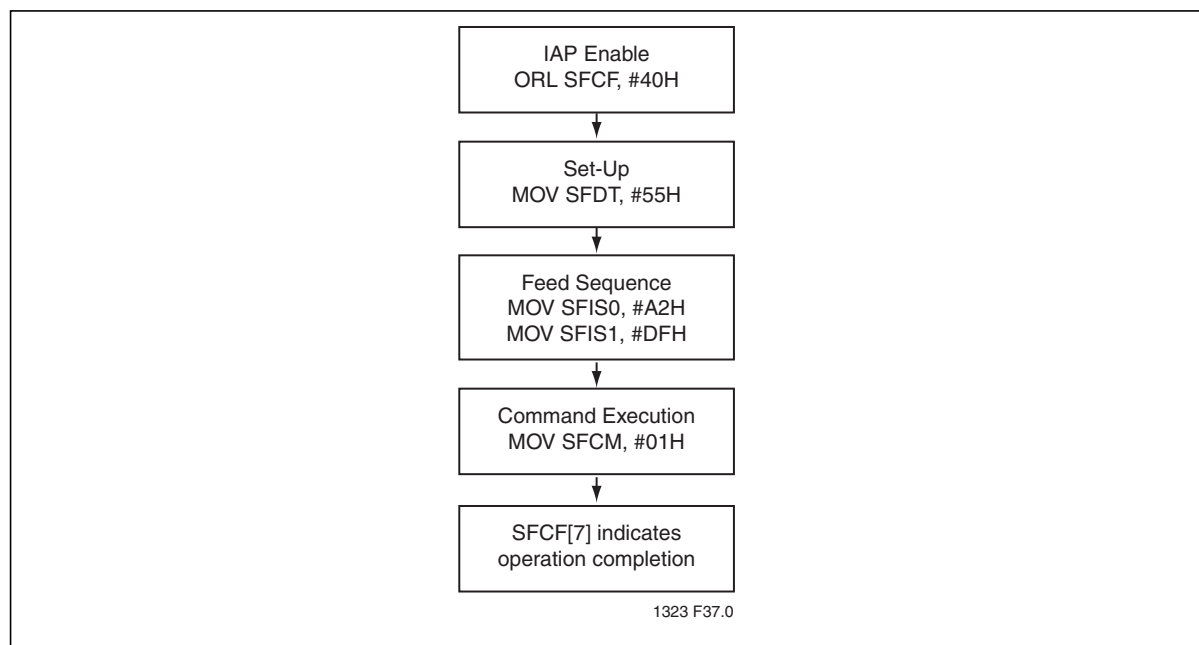
Figure 8: Chip-Erase
