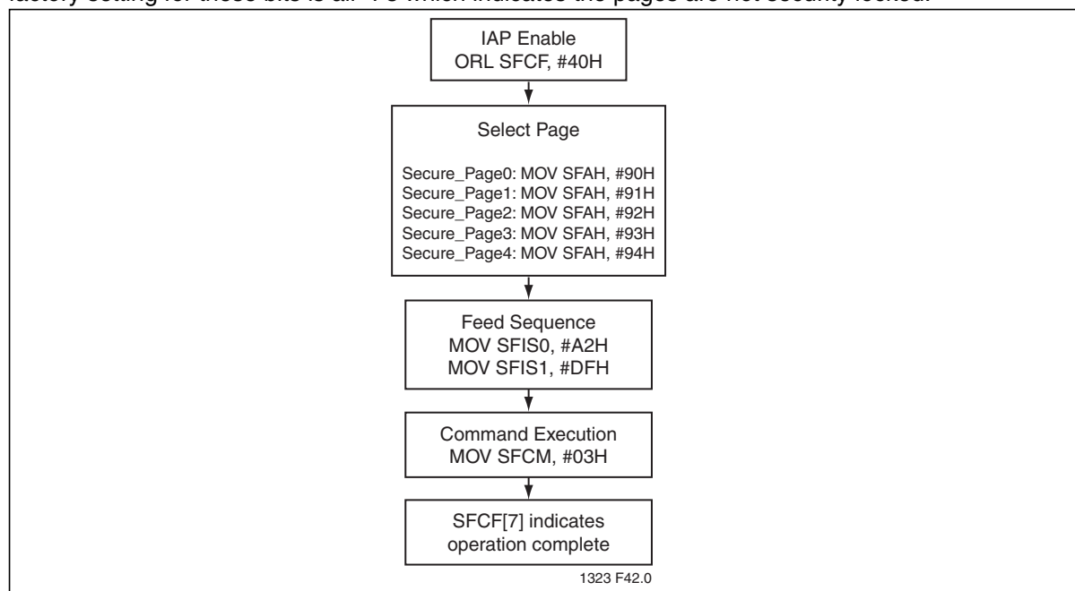
Figure 13: Secure-Page0-4
