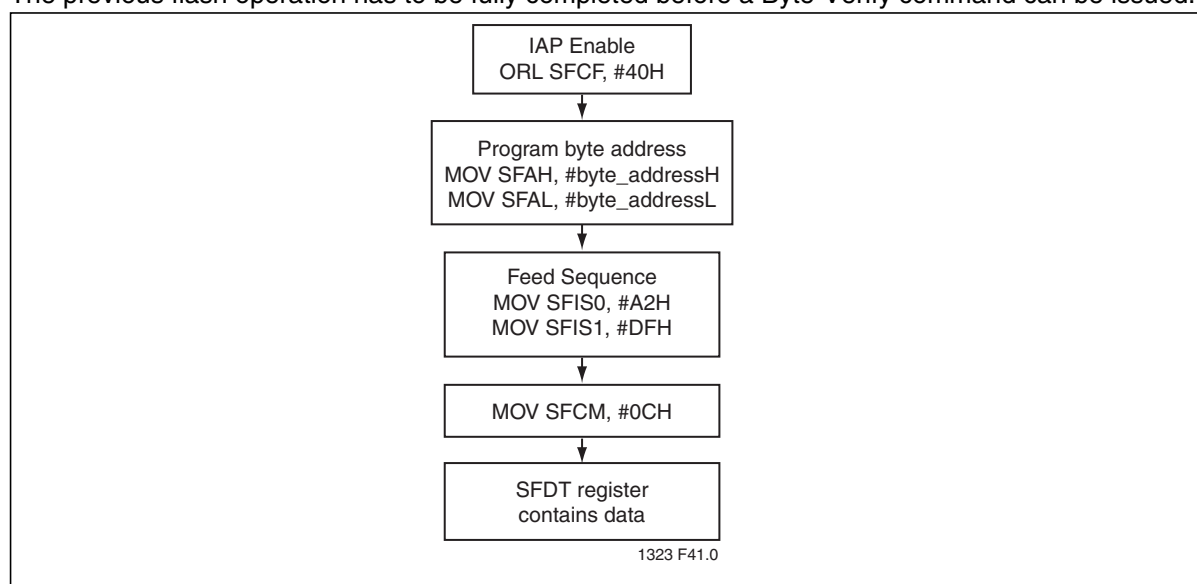
Figure 12: Byte-Verify
