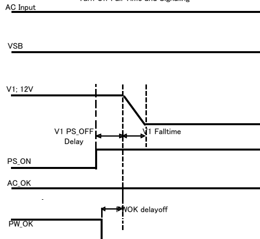
Turn Off Fall Time and Signaling
