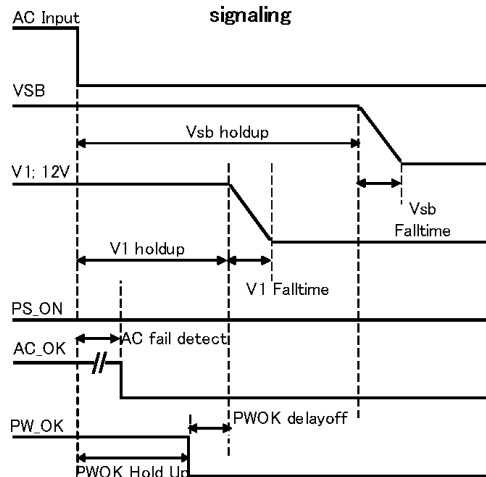
Power removed holdup faltime and signaling
