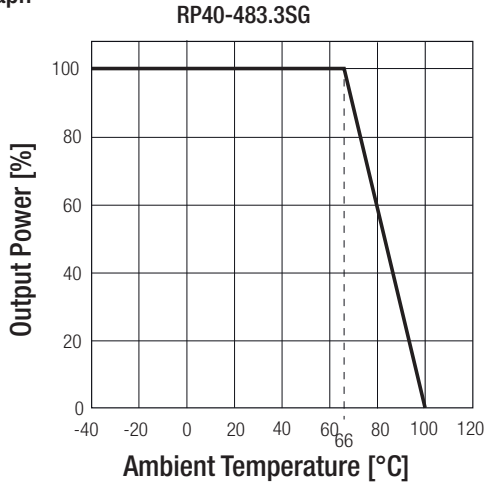
Derating Graph (10)
