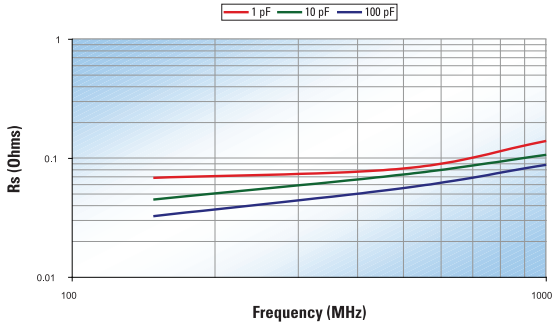
ESR vs Frequency DLI C11 AH Series
