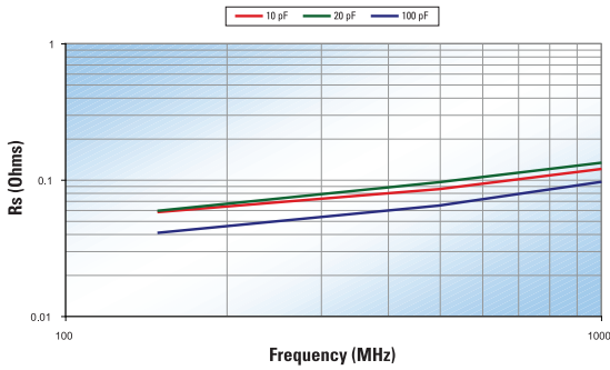
ESR vs Frequency DLI C12 MS Series
