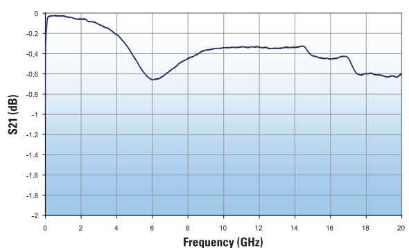
C04BL121X-5UN-X0T Insertion Loss (S21)
