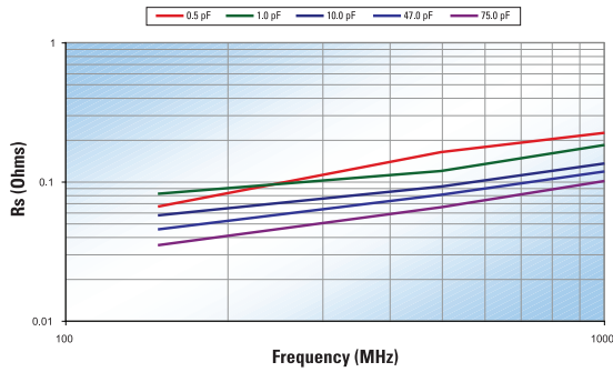
ESR vs Frequency DLI C06 MS Series
