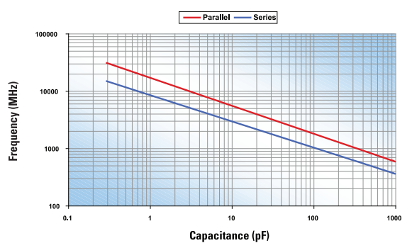
Resonant Frequency vs Capacitance DLI C17 MS Series
