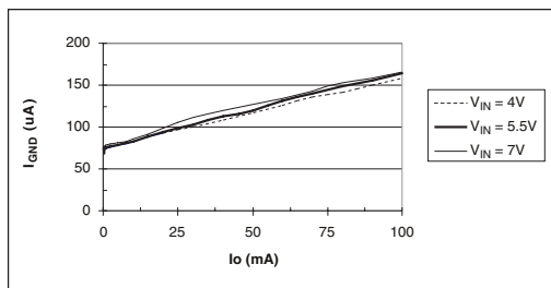
Ground Current vs. Output Current
