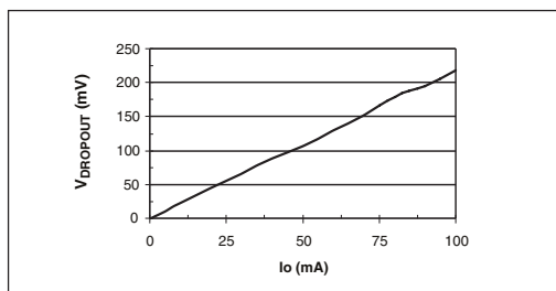
Dropout Voltage vs. Output Current
