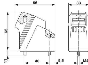
Dimensional drawing
