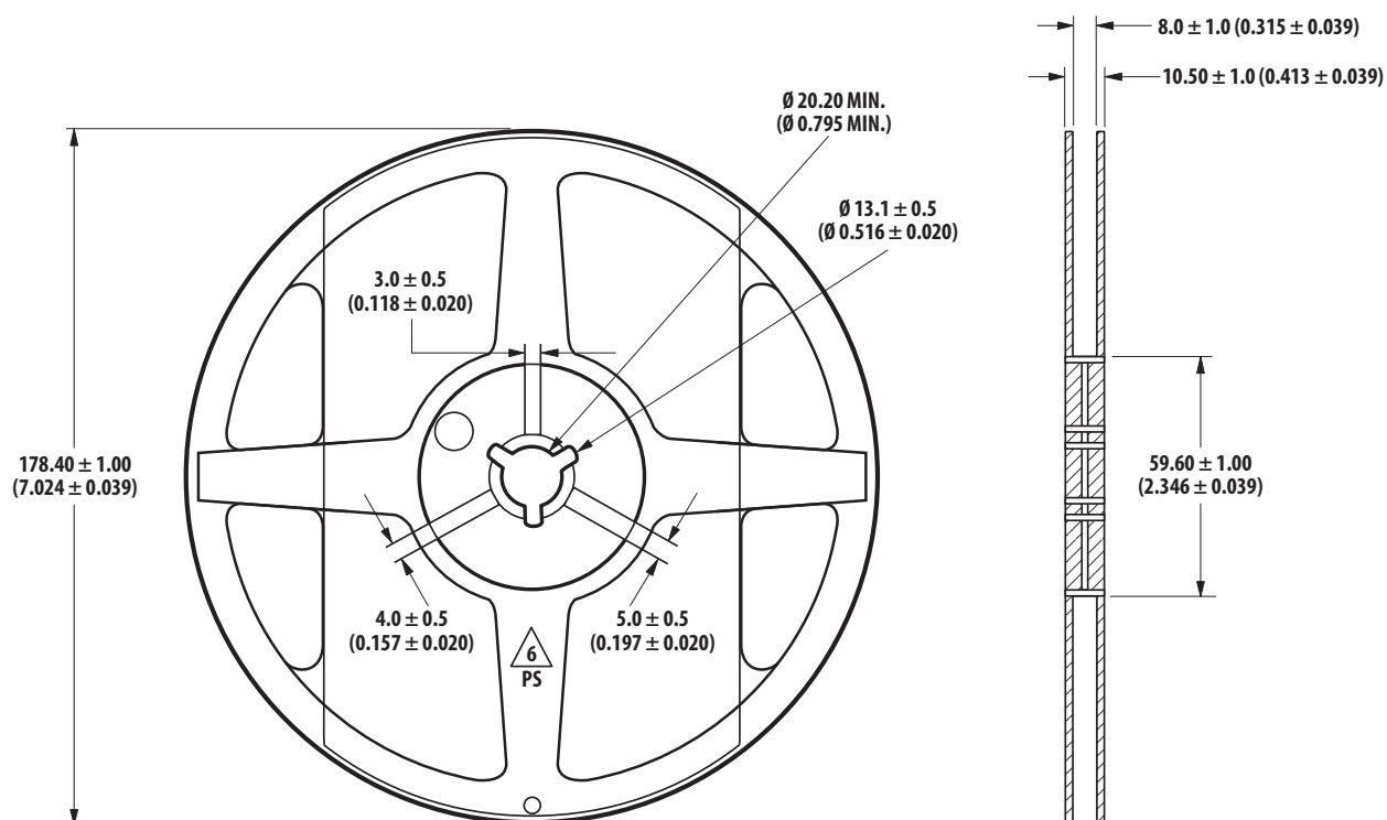
Figure 8: Reel Dimensions
