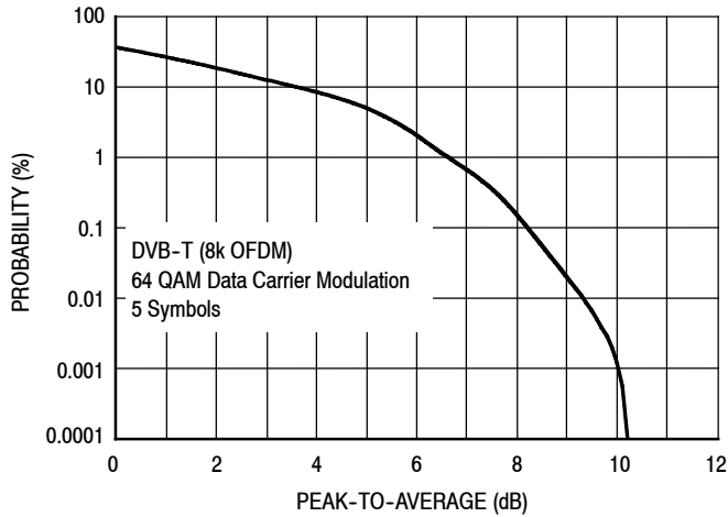
Figure 13. Single-Carrier DVB-T (8k OFDM)
