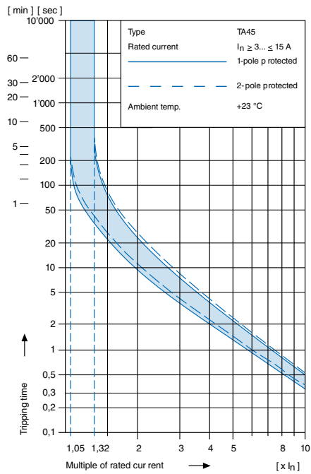
Tripping Characteristics I_n \ge 3 \dots \le 15 A
