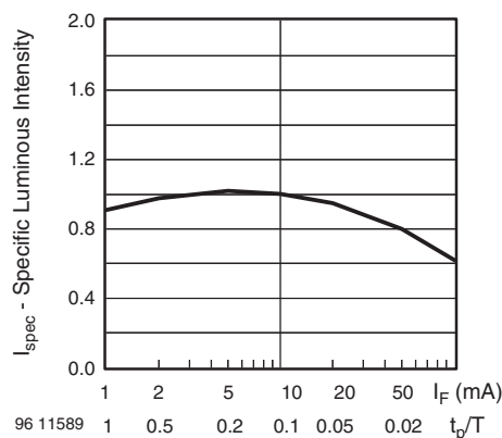
Fig. 5 - Specific Luminous Intensity vs. Forward Current/Duty Cycle
