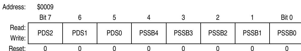
Figure 15-18. ESCI Prescaler Register (SCPSC)
