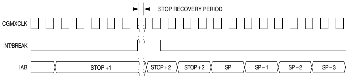
Figure 16-19. Stop Mode Recovery from Interrupt
