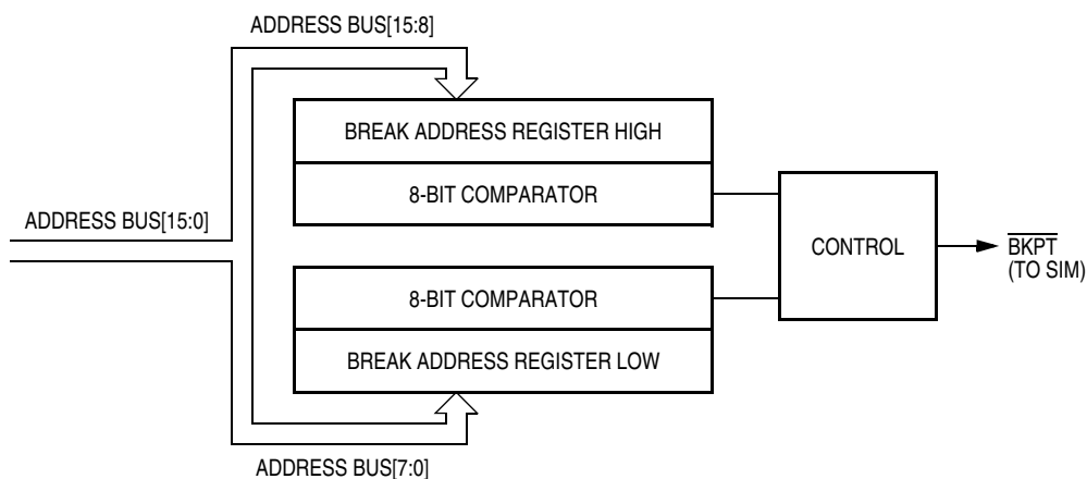
Figure 20-1. Break Module Block Diagram
