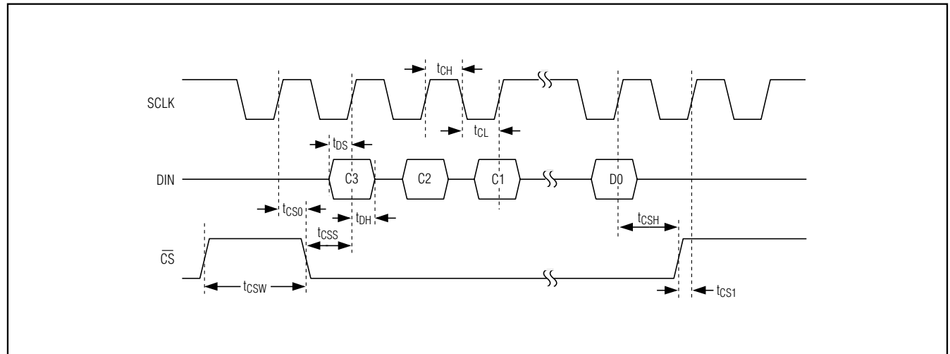
Figure 1. Timing Diagram
