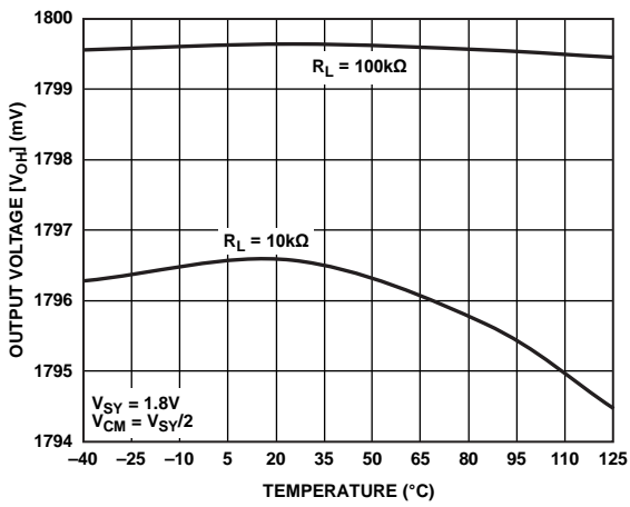
Figure 18. Output Voltage (V OH ) vs. Temperature
